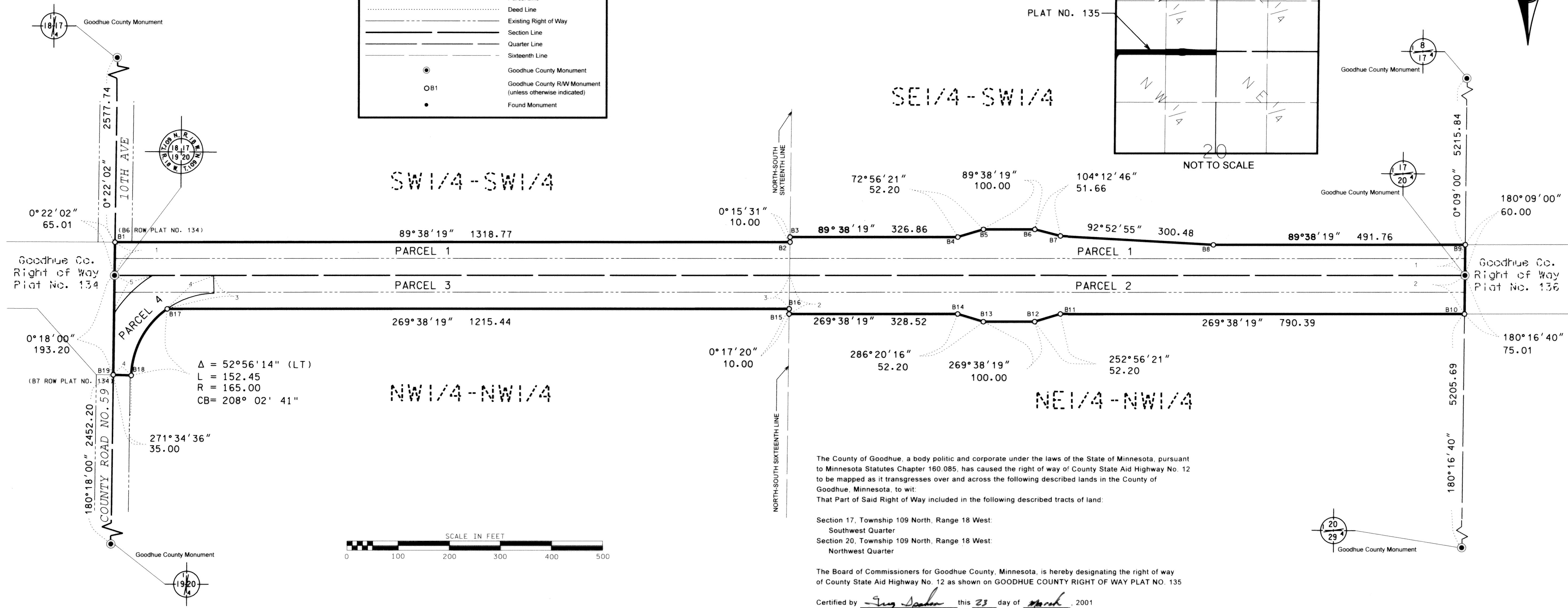
Right of Way in Section 17 and 20 T.109N., R.18W
